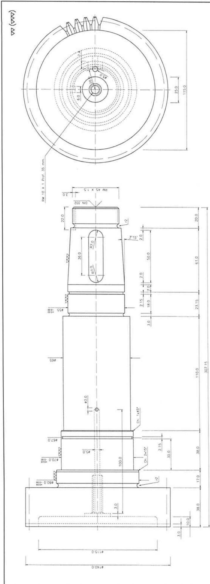
VISTA FRONTAL
