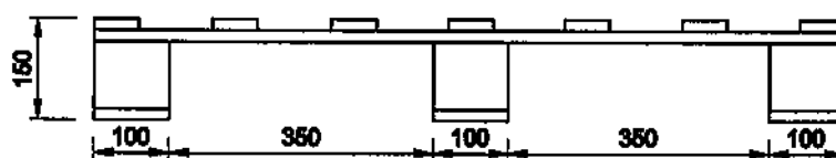
VISTA FRONTAL
