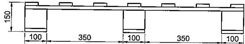
VISTA FRONTAL
