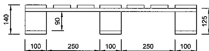
VISTA FRONTAL
